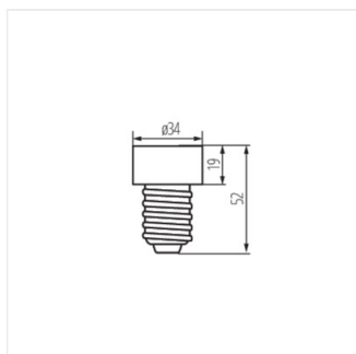
HLDR-E27/GU10
